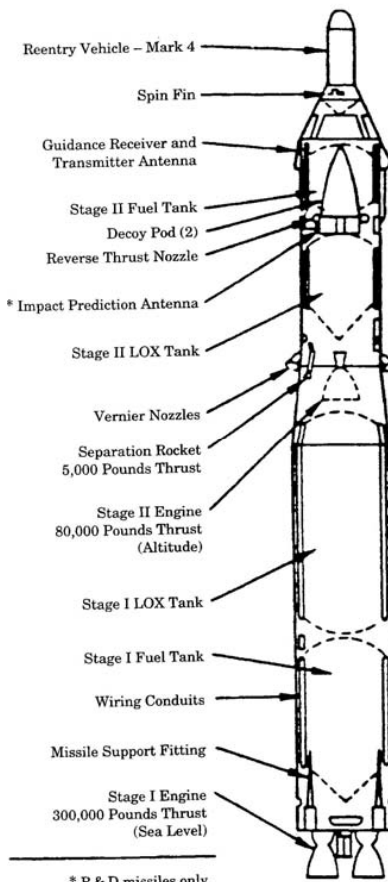
Plate 7. Drawing of Titan I, the United States' first two-stage ICBM ( Lonnquest and Winkler, To Defend and Deter: The Legacy of the United States Cold War Missile Program , 228)
