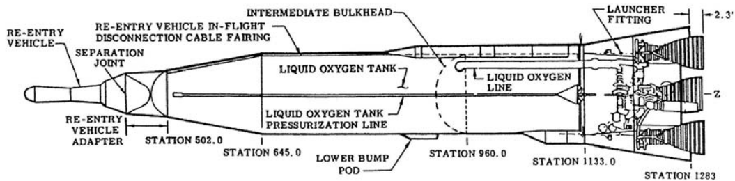
Plate 6. Cutaway drawing of an Atlas D ICBM. Later Atlas E and F missiles used the same airframe but added more powerful engines ( John C. Lonnquest and David F. Winkler, To Defend and Deter: The Legacy of the United States Cold War Missile Program (Washington, D.C.: Department of Defense, Legacy Resource Management Program, 1996), 210)
